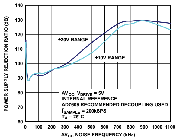
Figure 30. PSRR
