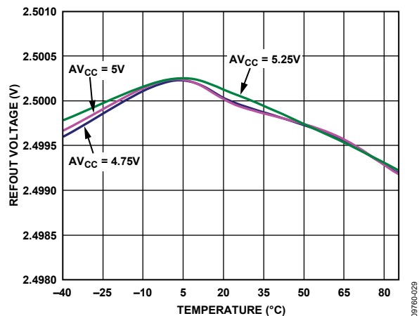
Figure 27. Reference Output Voltage vs. Temperature for Different Supply Voltages
