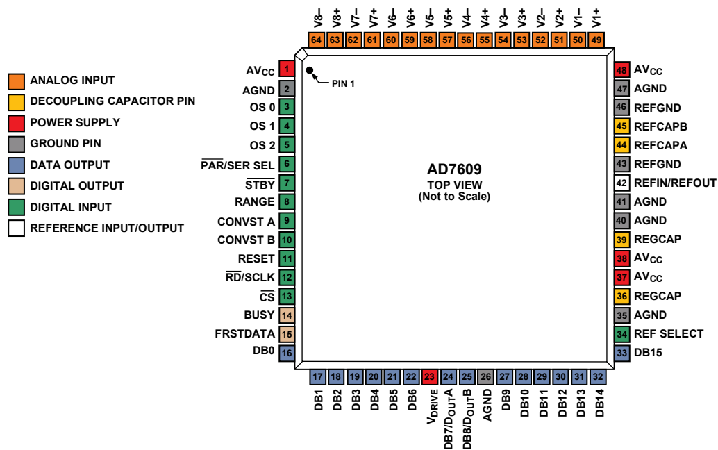
Figure 7. Pin Configuration
