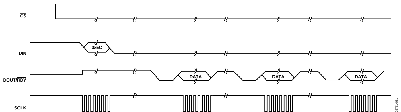
Figure 23. Continuous Read
