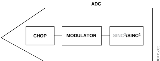
Figure 40. Chop Enabled
