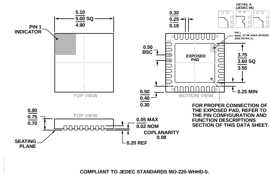
Figure 68. 32-Lead Lead Frame Chip Scale Package [LFCSP] 5 mm × 5 mm Body and 0.75 mm Package Height (CP-32-12) Dimensions shown in millimeters
