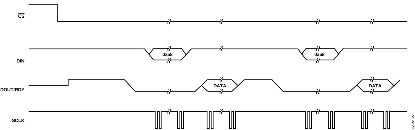
Figure 30. Continuous Conversion
