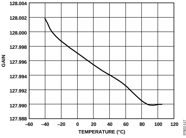
Figure 17. Gain Error (Gain = 128)
