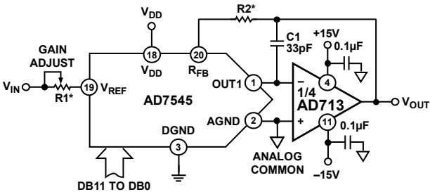
*REFER TO TABLE 5. Figure 42. Unipolar Binary Operation
