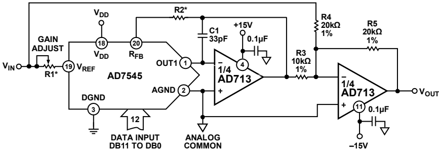
*REFER TO TABLE 5. Figure 43. Bipolar Operation
