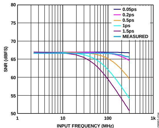
Figure 34. SNR vs. Input Frequency and Jitter
