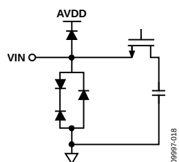
Figure 18. Equivalent Analog Input Circuit
