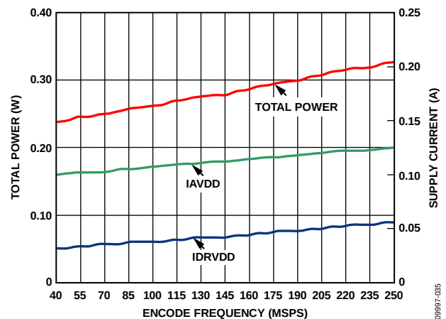
Figure 35. AD6672-250 Power and Current vs. Sample Rate
