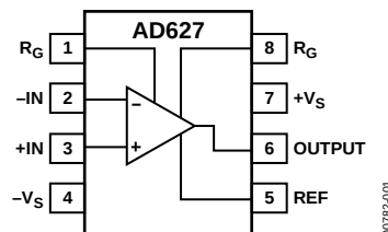
Figure 1. 8-Lead PDIP (N) and SOIC_N (R)
