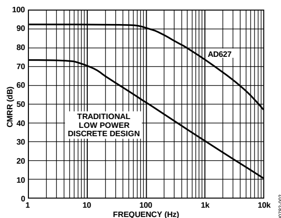
Figure 2. CMRR vs. Frequency, \pm 5 V, Gain = +5
