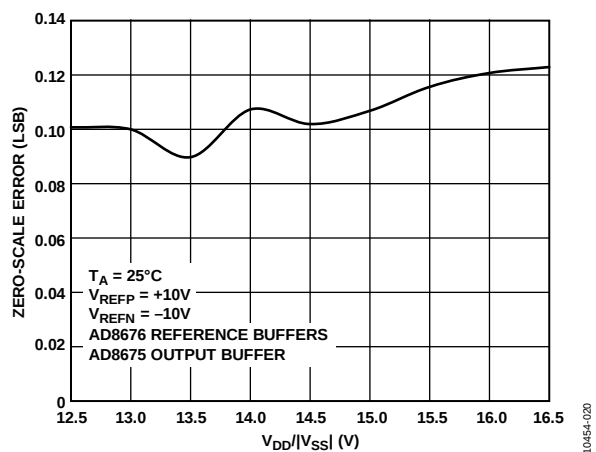
Figure 19. Zero-Scale Error vs. Supply Voltage, \pm 10\text{ V Span}
