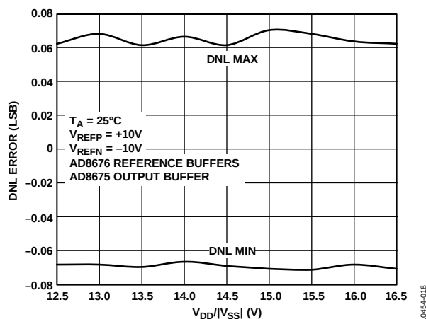
Figure 17. Differential Nonlinearity Error vs. Supply Voltage, \pm 10\text{ V Span}
