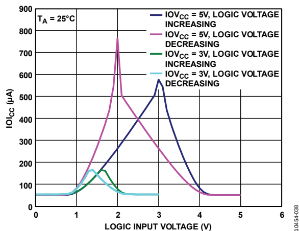
Figure 37. I_{OI} vs. Logic Input Voltage
