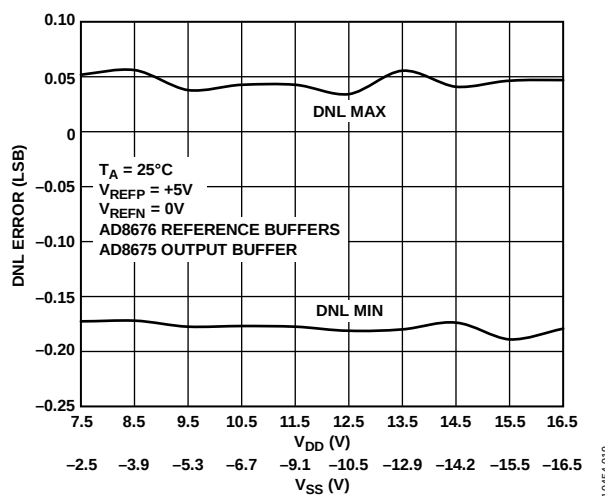
Figure 18. Differential Nonlinearity Error vs. Supply Voltage, +5\text{ V Span}
