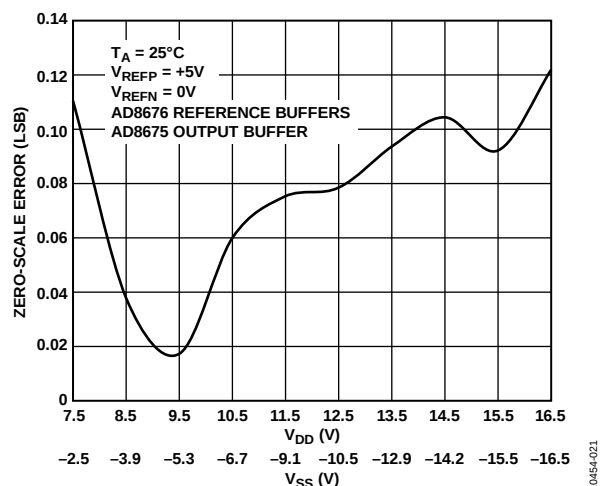
Figure 20. Zero-Scale Error vs. Supply Voltage, +5\text{ V Span}
