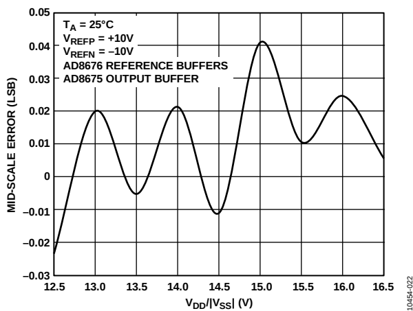
Figure 21. Midscale Error vs. Supply Voltage, \pm 10\text{ V Span}
