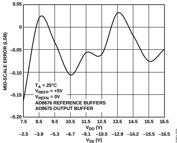
Figure 22. Midscale Error vs. Supply Voltage, +5\text{ V Span}
