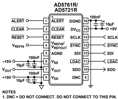
Figure 76. Typical Operating Circuit
