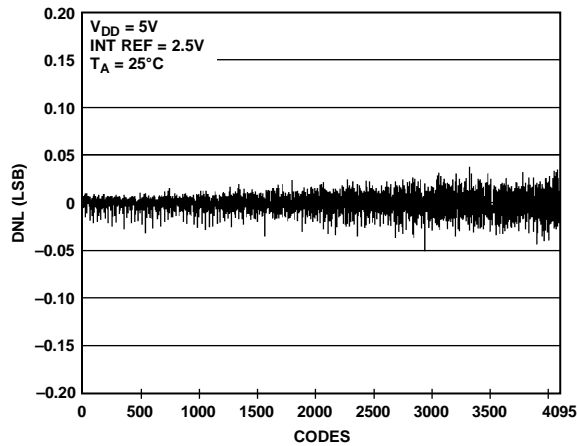
Figure 13. DNL AD5629R-2—Internal Reference
