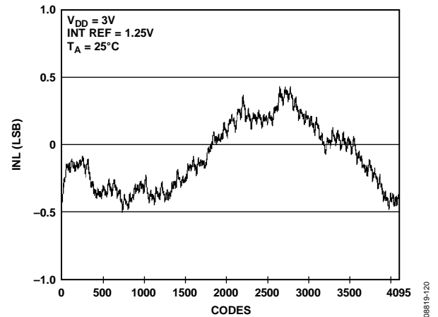
Figure 15. INL AD5669R-1—Internal Reference
