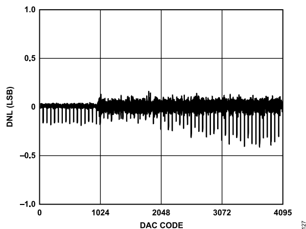
Figure 14. DAC DNL
