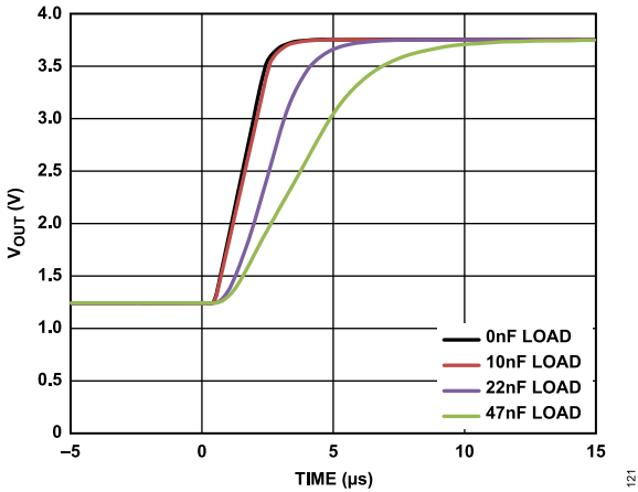
Figure 22. DAC Settling Time vs. Capacitive Load
