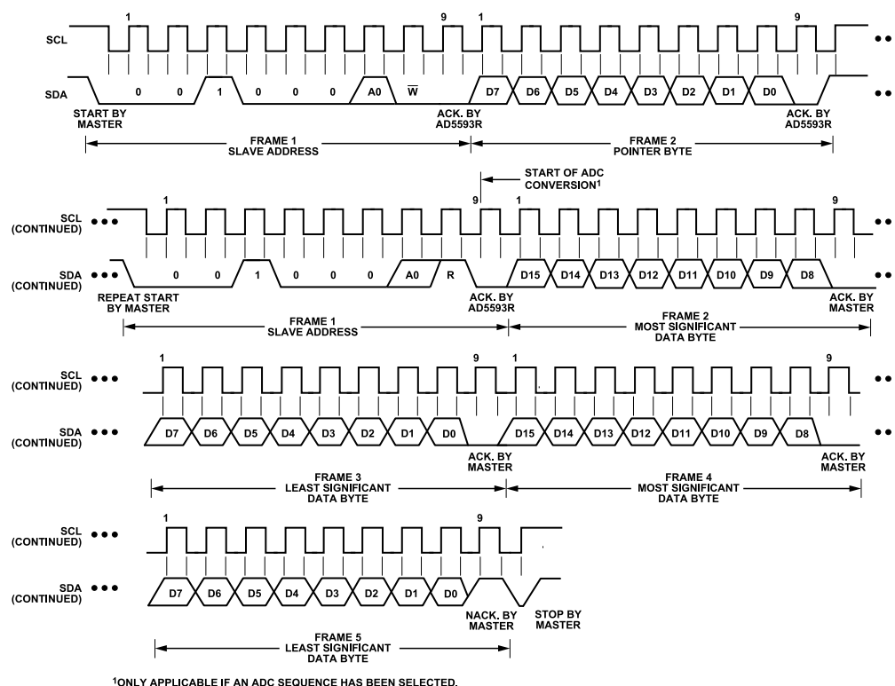
Figure 39. I²C Block Read
