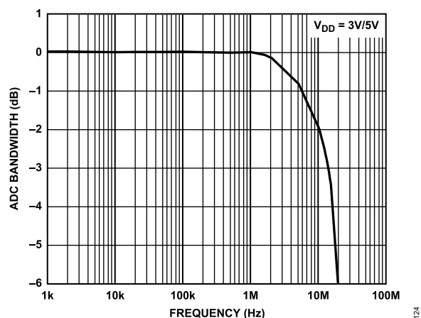
Figure 12. ADC Bandwidth
