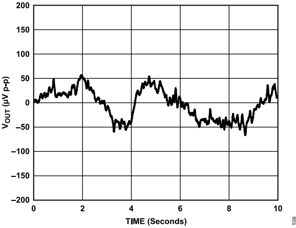
Figure 23. DAC 1/f Noise with External Reference
