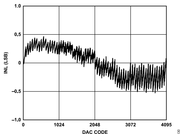
Figure 13. DAC INL
