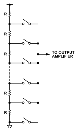
Figure 32. Resistor String
