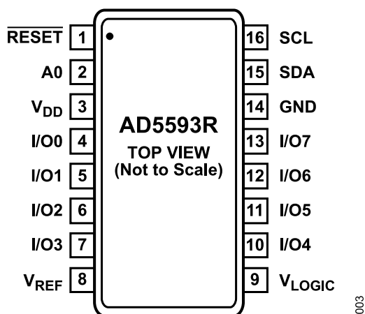
Figure 3. 16-Lead TSSOP Pin Configuration
