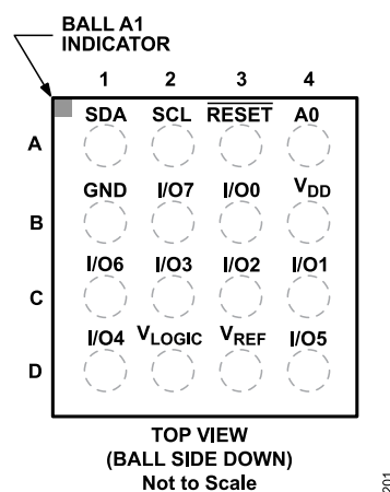
Figure 5. 16-Ball WLCSP Pin Configuration
