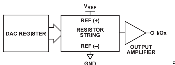
Figure 31. DAC Channel Architecture Block Diagram
