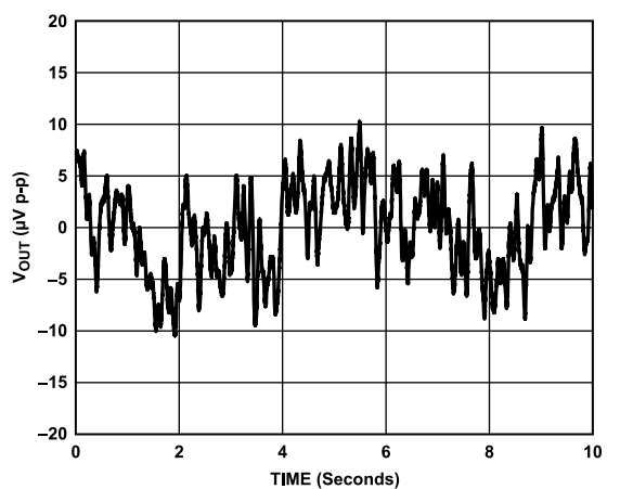
Figure 28. Internal Reference 1/f Noise
