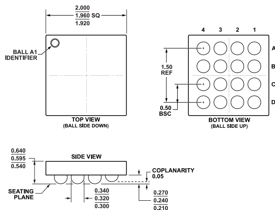
Figure 46. 16-Ball Wafer Level Chip Scale Package [WLCSOP] (CB-16-3) Dimensions shown in millimeters
