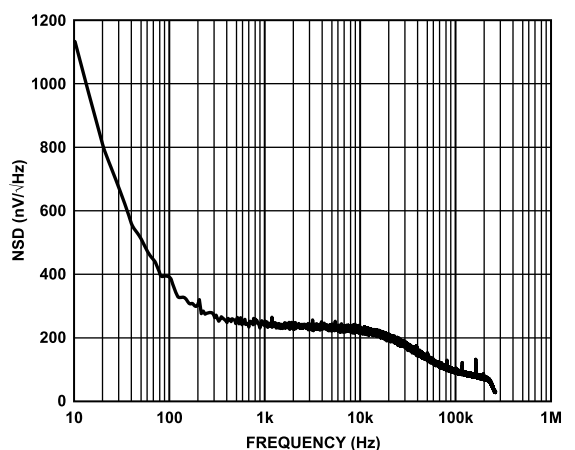
Figure 29. Reference Noise Spectral Density
