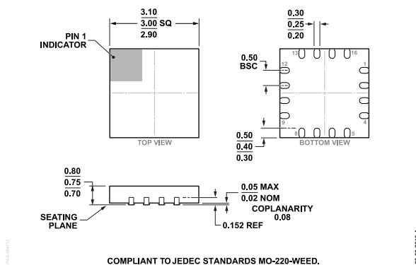
Figure 45. 16-Lead Lead Frame Chip Scale Package [LFCSOP] 3 mm × 3 mm Body and 0.75 mm Package Height (CP-16-32) Dimensions shown in millimeters
