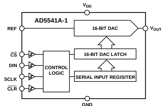
Figure 2. AD5541A-1
