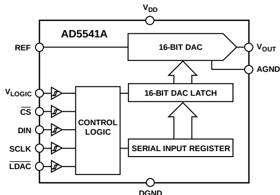
Figure 1. AD5541A
