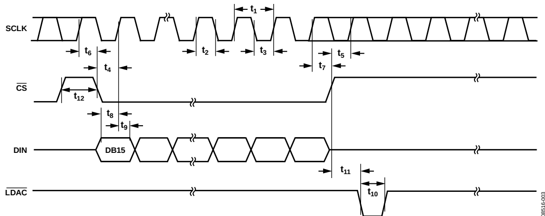
Figure 3. Timing Diagram
