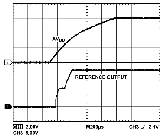
Figure 28. Reference Turn-on Transient
