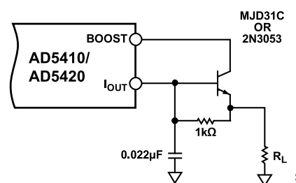
Figure 41. External Boost Configuration
