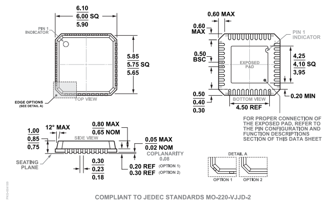
Figure 57. 40-Lead Lead Frame Chip Scale Package [LFCSP] (CP-40-1) 6 mm × 6 mm Body and 0.85 mm Package Height Dimensions shown in millimeters
