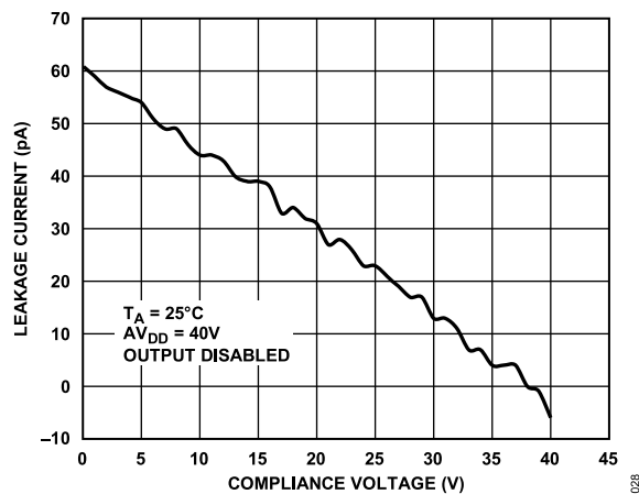
Figure 31. Output Leakage Current vs. Compliance Voltage
