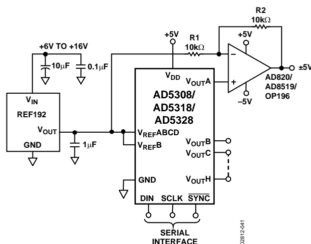
Figure 41. Bipolar Operation with the AD5308/AD5318/AD5328
