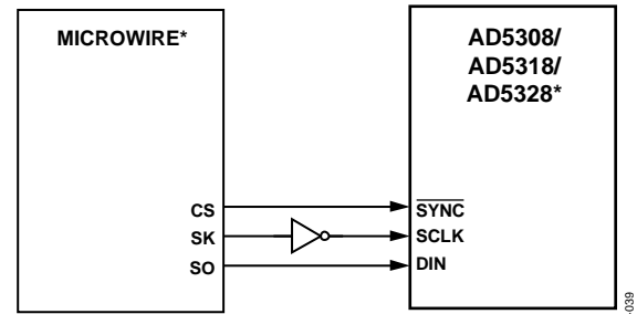
Figure 39. MICROWIRE-to-AD5308/AD5318/AD5328 Interface
