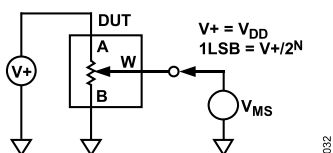
Figure 32. Potentiometer Divider Nonlinearity Error (INL, DNL)
