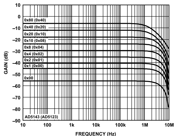
Figure 20. 100 kΩ Gain vs. Frequency and Code
