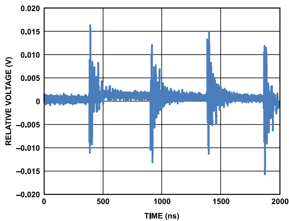
Figure 28. Digital Feedthrough
