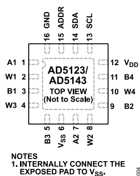
Figure 4. Pin Configuration
