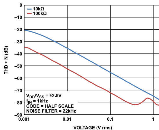
Figure 21. Total Harmonic Distortion Plus Noise (THD + N) vs. Amplitude
