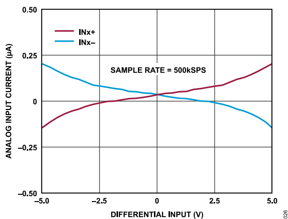
Figure 26. Analog Input Current vs. Differential Input, AD4630-24, 500 kSPS
