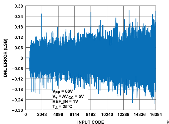
Figure 5. DNL with Full-Scale Range = 50 V
