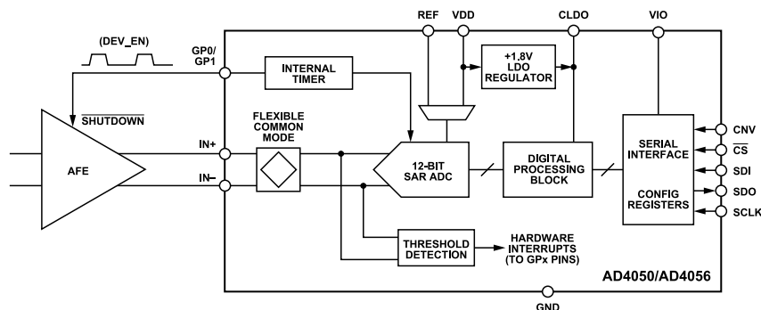
Figure 33. AD4050/AD4056 Functional Block Diagram
