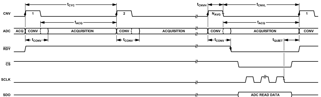
Figure 49. Averaging Mode Timing Diagram
