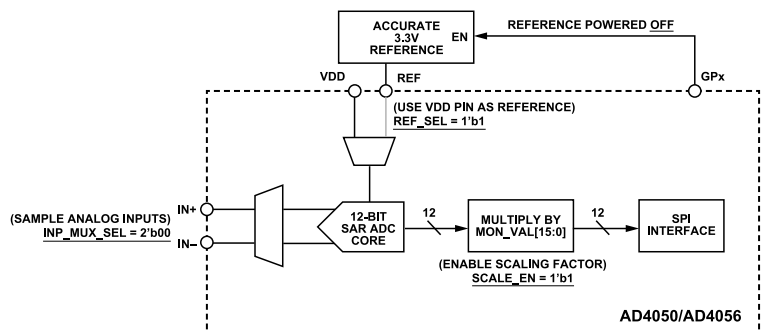
Figure 74. MON_VAL Application Configuration
