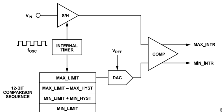
Figure 39. Simplified Schematic of Autonomous Mode Window Comparator
