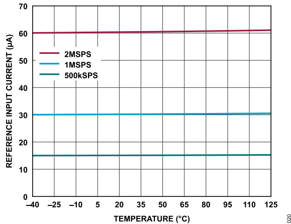
Figure 20. Reference Input Current vs. Temperature
