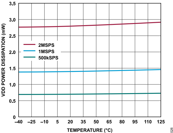
Figure 26. VDD Power Dissipation vs. Temperature
