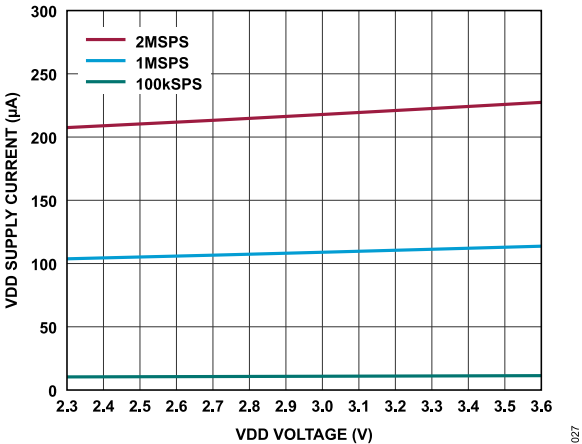
Figure 27. VDD Supply Current vs. VDD Voltage (Autonomous Modes)
