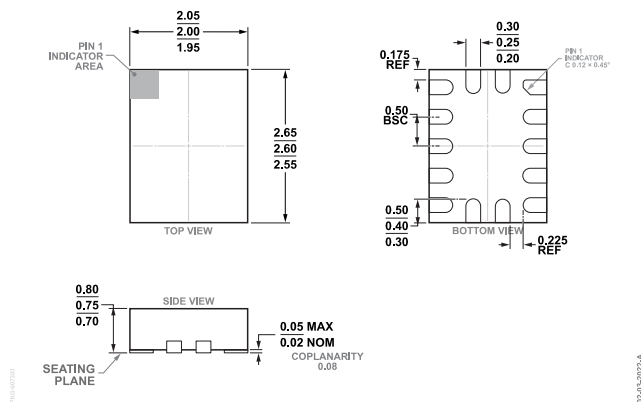
Figure 78. 14-Lead Lead Frame Chip Scale Package [LFCSP] 2 mm × 2.6 mm Body and 0.75 mm Packaging Height (CP-14-7) Dimensions shown in millimeters
