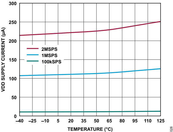
Figure 28. VDD Supply Current vs. Temperature (Autonomous Modes)
