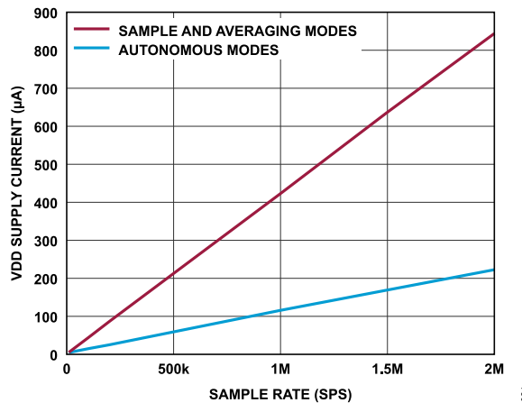
Figure 21. VDD Supply Current vs. Sample Rate
