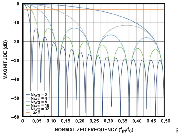
Figure 38. Frequency Response Examples for the Block Averaging Filter
