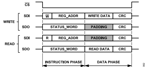
Figure 62. Configuration Mode SPI Format
