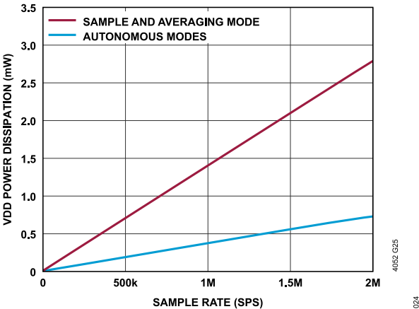
Figure 24. VDD Power Dissipation vs. Sample Rate
