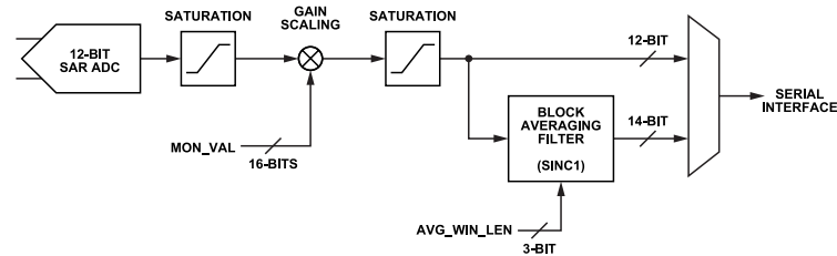
Figure 37. AD4050/AD4056 Digital Processing Functionality
