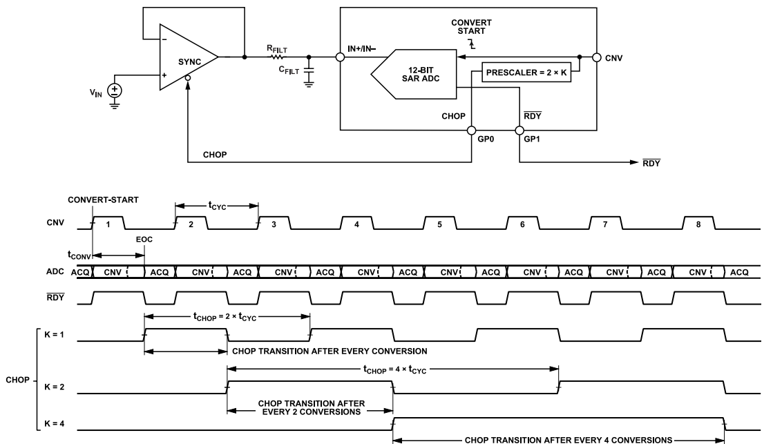
Figure 42. Typical Application Circuit with CHOP Signal
