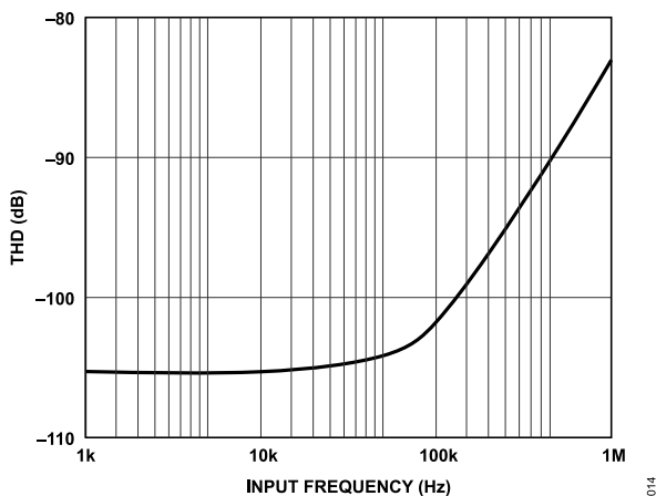
Figure 14. THD vs. Input Frequency, V_{IN} = -1\text{dBFS}
