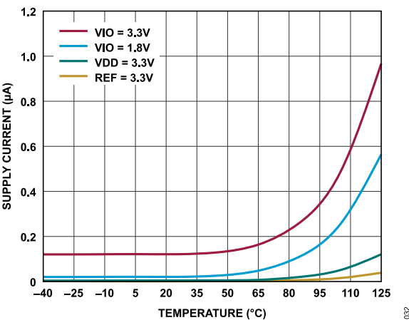
Figure 32. Supply Current (Sleep Mode) vs. Temperature
