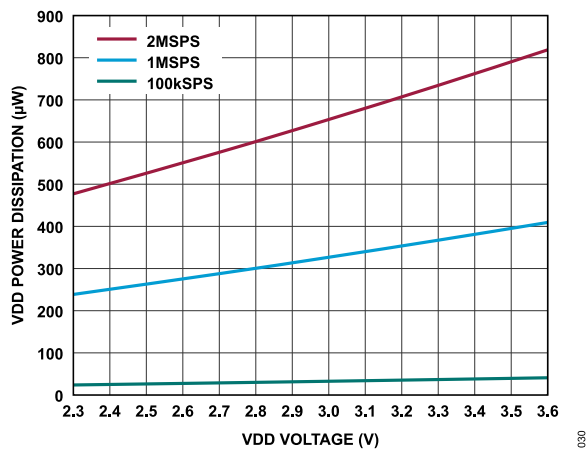
Figure 30. VDD Power Dissipation vs. VDD Voltage (Autonomous Modes)
