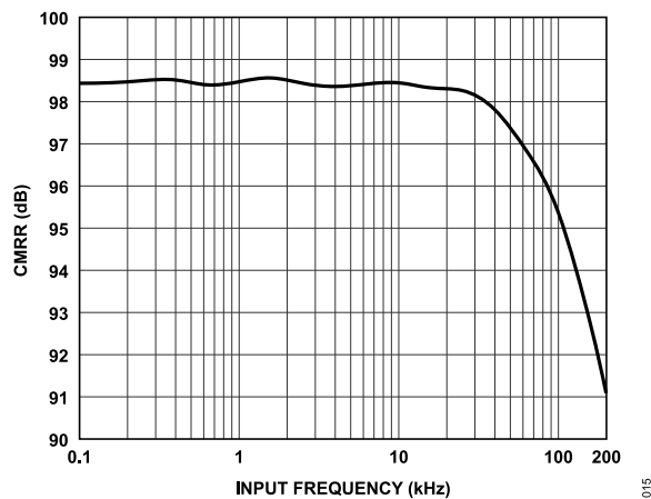
Figure 15. Common-Mode Rejection Ratio (CMRR) vs. Input Frequency
