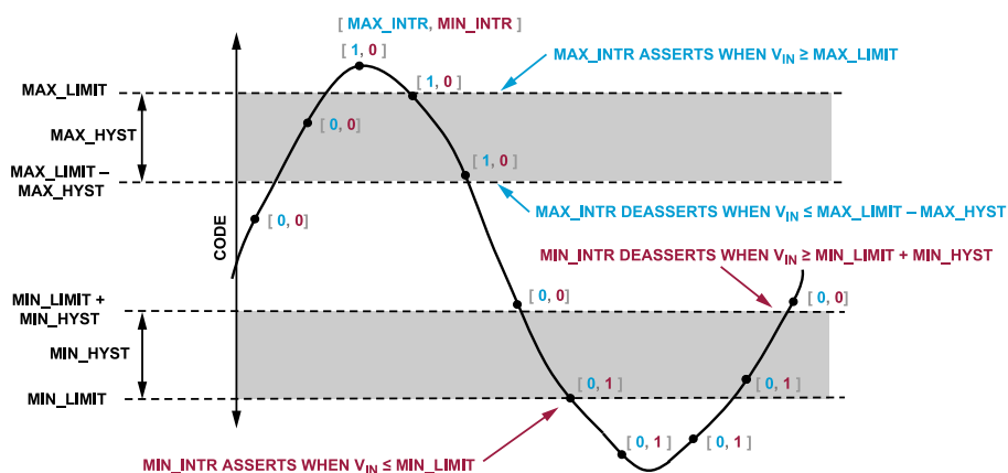
Figure 40. Threshold Event Regions
