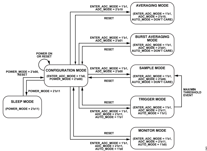
Figure 45. AD4050/AD4056 State Machine Diagram
