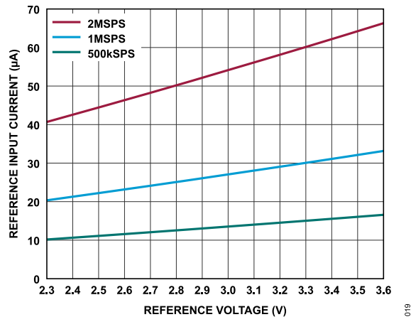
Figure 19. Reference Input Current vs. Reference Voltage
