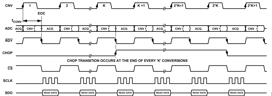
Figure 55. Sample Mode Timing with CHOP Enabled
