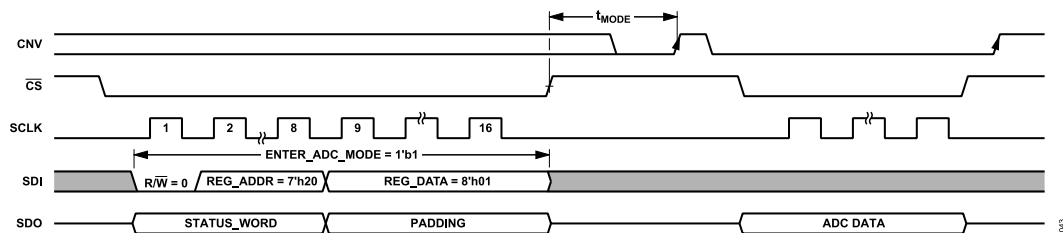
Figure 43. ENTER_ADC_MODE Timing Diagram
