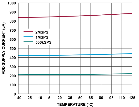
Figure 23. VDD Supply Current vs. Temperature
