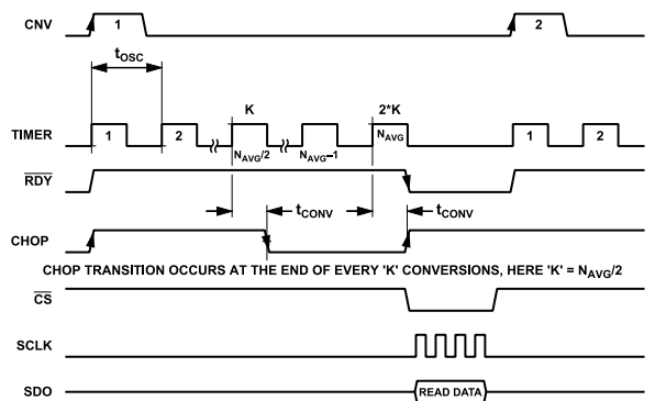
Figure 57. Burst Averaging Mode Timing with CHOP Enabled
