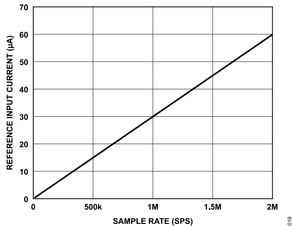
Figure 18. Reference Input Current vs. Sample Rate
