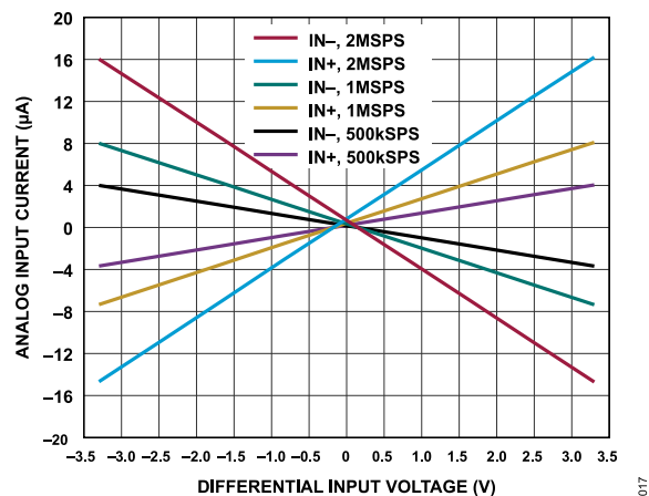
Figure 17. Analog Input Current vs. Differential Input Voltage
