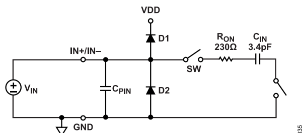
Figure 35. Equivalent Analog Input Circuit
