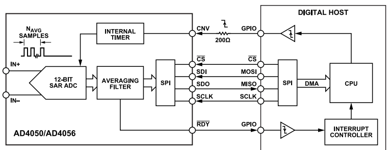
Figure 50. Burst Averaging Mode Example Connection Diagram
