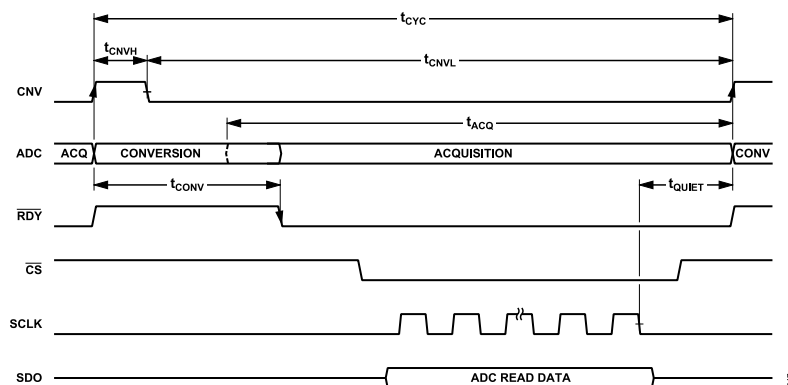
Figure 47. Sample Mode Timing Diagram
