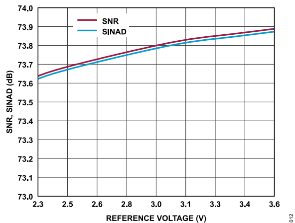
Figure 12. SNR, SINAD vs. Reference Voltage
