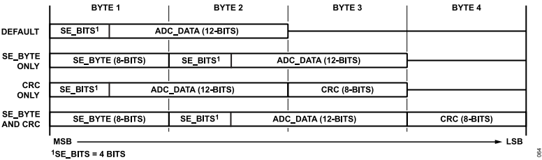
Figure 64. SPI Data Formats for Sample Mode and Trigger Mode
