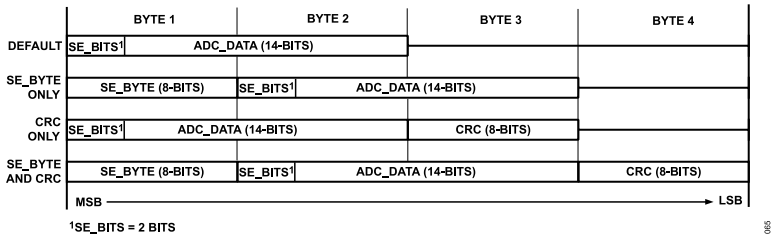
Figure 65. SPI Data Formats for Averaging Mode and Burst Averaging Mode
