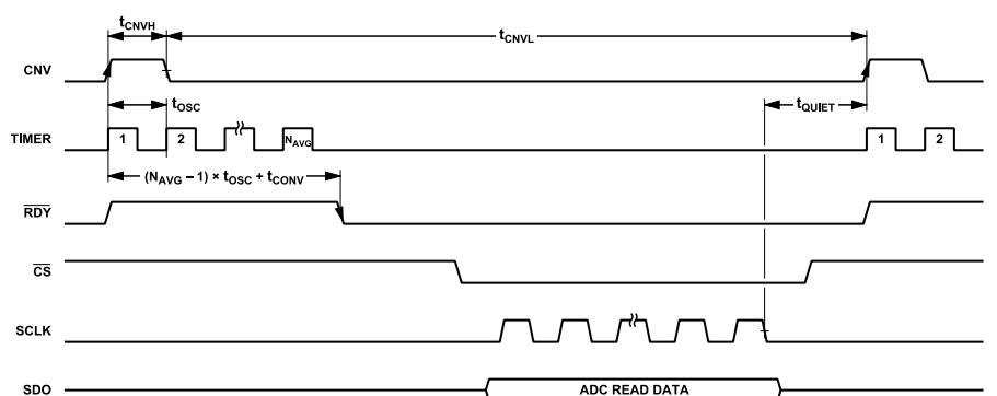
Figure 51. Burst Averaging Mode Timing Diagram
