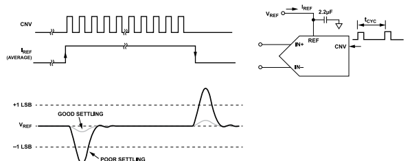
Figure 72. Burst Sampling and Voltage Reference Settling
