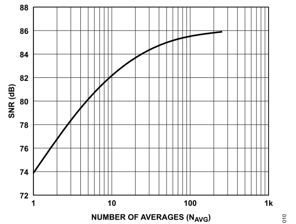
Figure 10. SNR vs. Number of Averages
