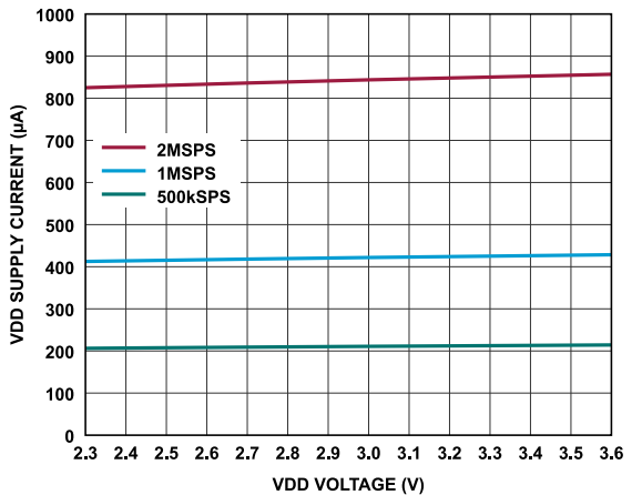
Figure 22. VDD Supply Current vs. VDD Voltage
