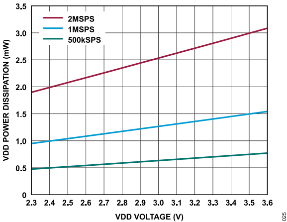
Figure 25. VDD Power Dissipation vs. VDD Voltage
