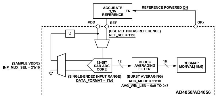
Figure 73. MON_VAL Calculation Configuration
