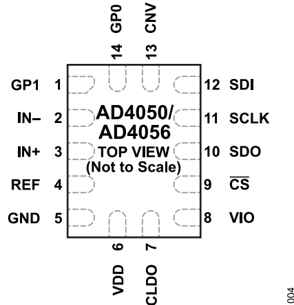
Figure 4. AD4050/AD4056 LFCSP Pin Configuration
