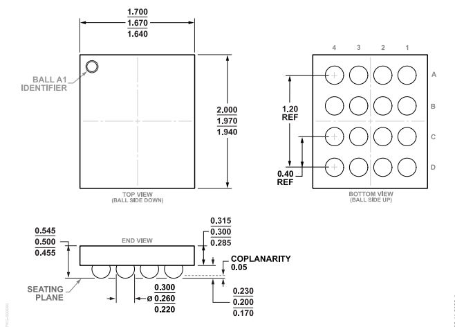
Figure 79. 16-Ball Wafer Level Chip Scale Package [WLCSP] (CB-16-26) Dimensions shown in millimeters
