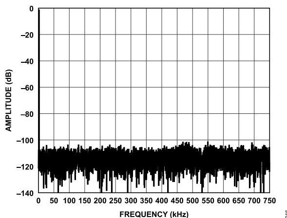
Figure 16. Fast Fourier Transform (FFT), f_S = 1.5\text{ MSPS} , f_{IN} = 1\text{ kHz}
