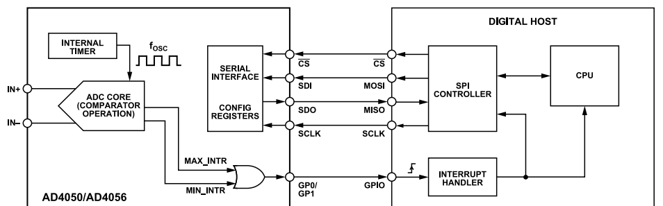
Figure 60. Autonomous Mode Example Connection Diagram
