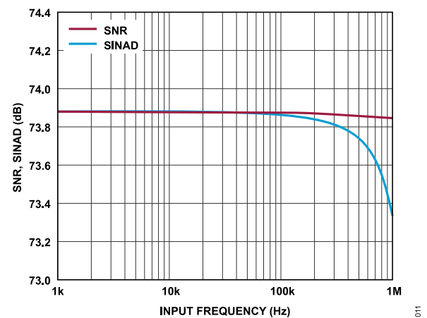
Figure 11. SNR, SINAD vs. Input Frequency
