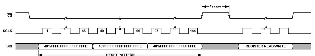
Figure 67. Reset Pattern Timing Diagram
