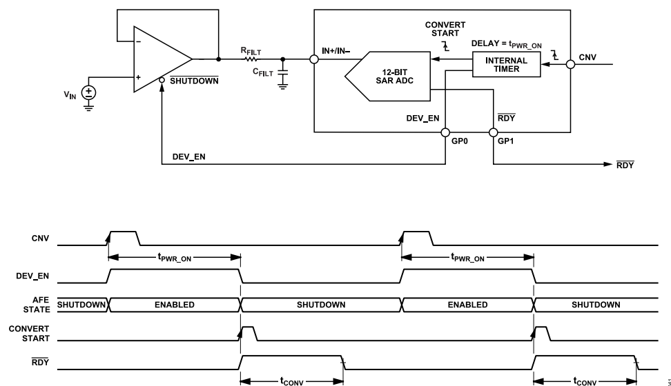
Figure 41. Typical Application Circuit with DEV_EN Signal
