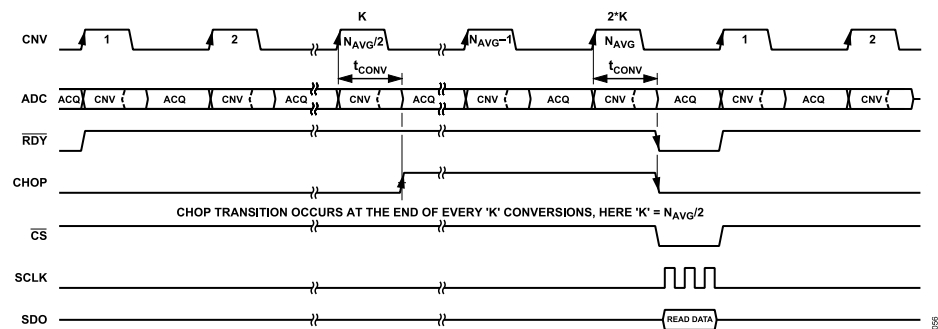
Figure 56. Averaging Mode Timing with CHOP Enabled
