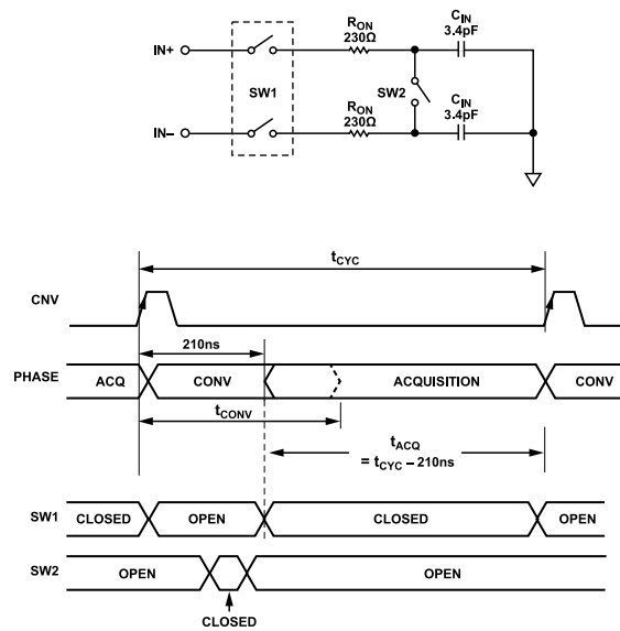
Figure 71. AD4050/AD4056 Equivalent Input Load Model
