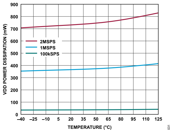
Figure 31. VDD Power Dissipation vs. Temperature (Autonomous Modes)
