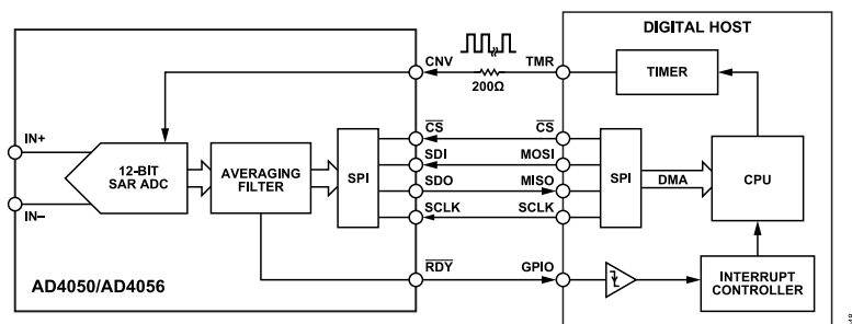
Figure 48. Averaging Mode Example Connection Diagram
