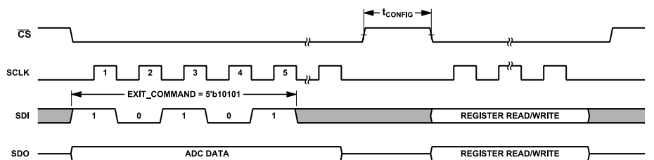
Figure 44. Exit Command Timing Diagram
