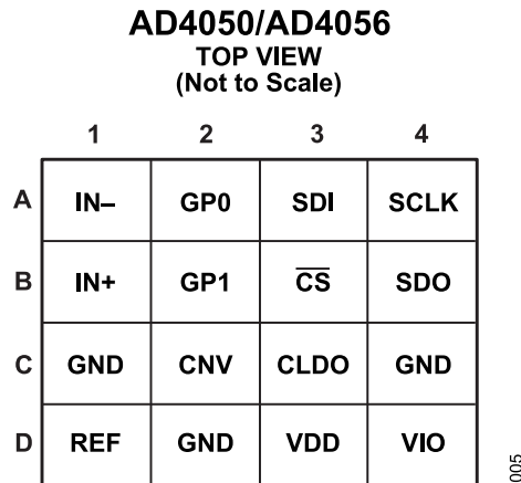
Figure 5. AD4050/AD4056 WLCSP Pin Configuration
