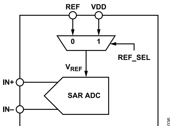
Figure 36. Reference Source Selection
