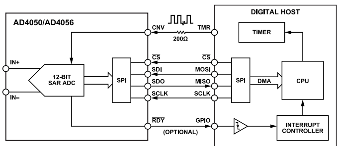
Figure 46. Sample Mode Example Connection Diagram
