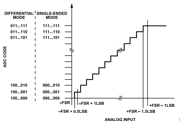
Figure 34. ADC Ideal Transfer Function
