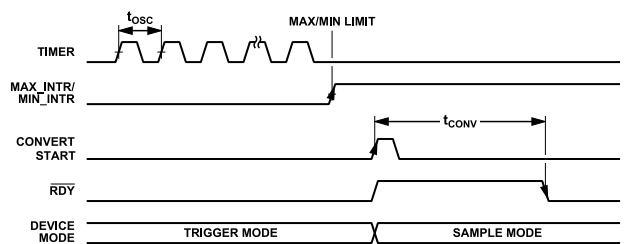
Figure 61. Trigger Mode Timing Diagram
