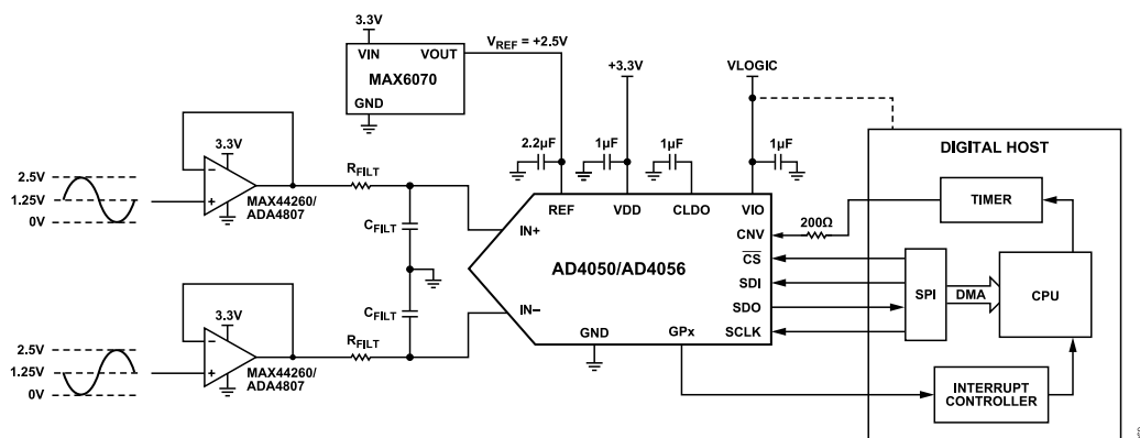
Figure 69. AD4050/AD4056 Typical Application Diagram
