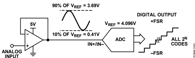
Figure 45. Span Compression
