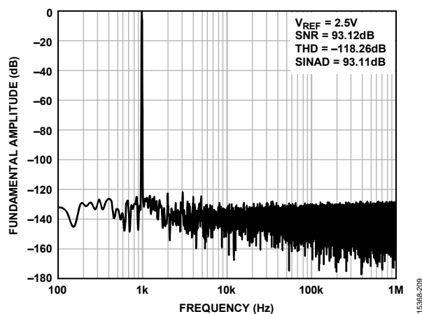
Figure 15. 1 kHz, -0.5 dBFS Input Tone FFT, V_{REF} = 2.5V
