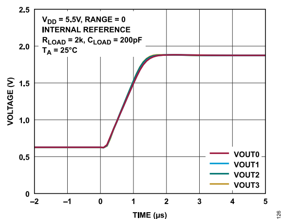
Figure 26. Settling Time
