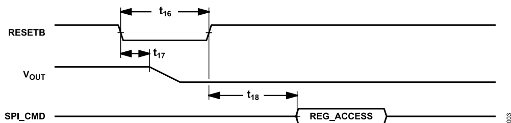
Figure 3. Reset Timing
