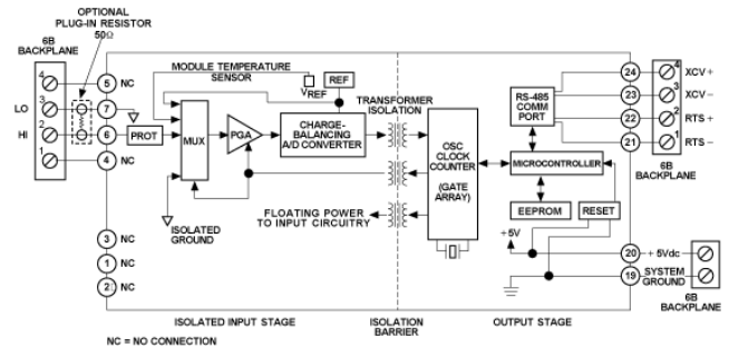
Figure 1. 6B12 & 6B12HV Functional Block Diagram
