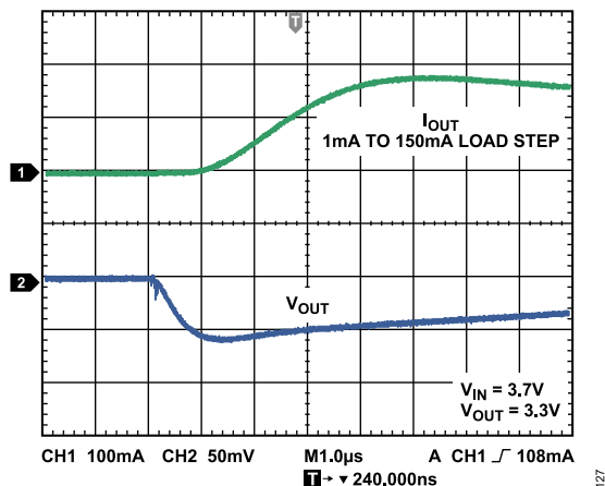
Figure 28. Output Transient Response, C_{OUT} = 4.7 \mu\text{F}
