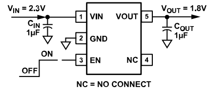
Figure 1. 5-Lead TSOT with Fixed Output Voltage, 1.8 V
