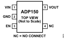
Figure 3. 5-Lead TSOT Pin Configuration
