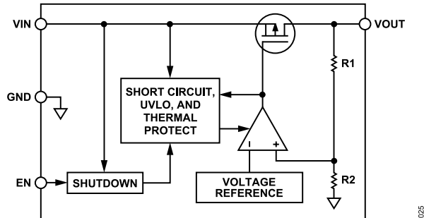
Figure 26. Internal Block Diagram
