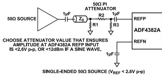
Figure 58. Single-Ended 50 Ω Source ( V REF < 2.6 V p-p)
