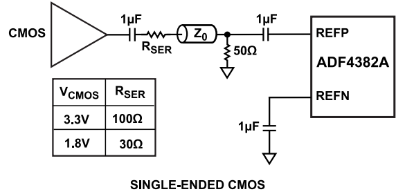
Figure 59. Single-Ended CMOS ( R SER Is the Series Resistance.)
