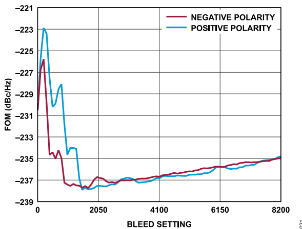
Figure 21. FOM, L_{1/f} Fractional Mode vs. Bleed Setting, f_{PFD} = 250 MHz, RFOUT = 20.001 GHz
