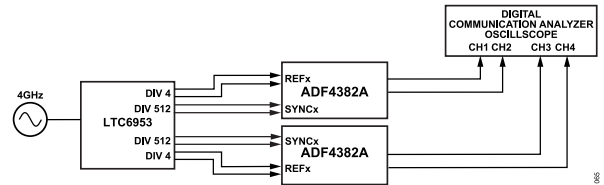
Figure 65. Timed Synchronization Configuration
