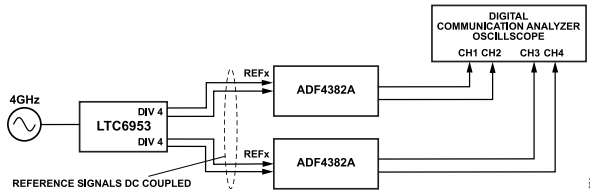
Figure 64. EZSync Configuration
