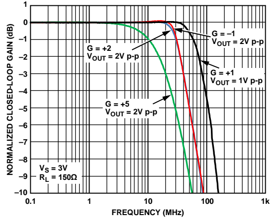
Figure 22. Large-Signal Frequency Response vs. Gain, V_S = 3V , ADA4891-3/ADA4891-4
